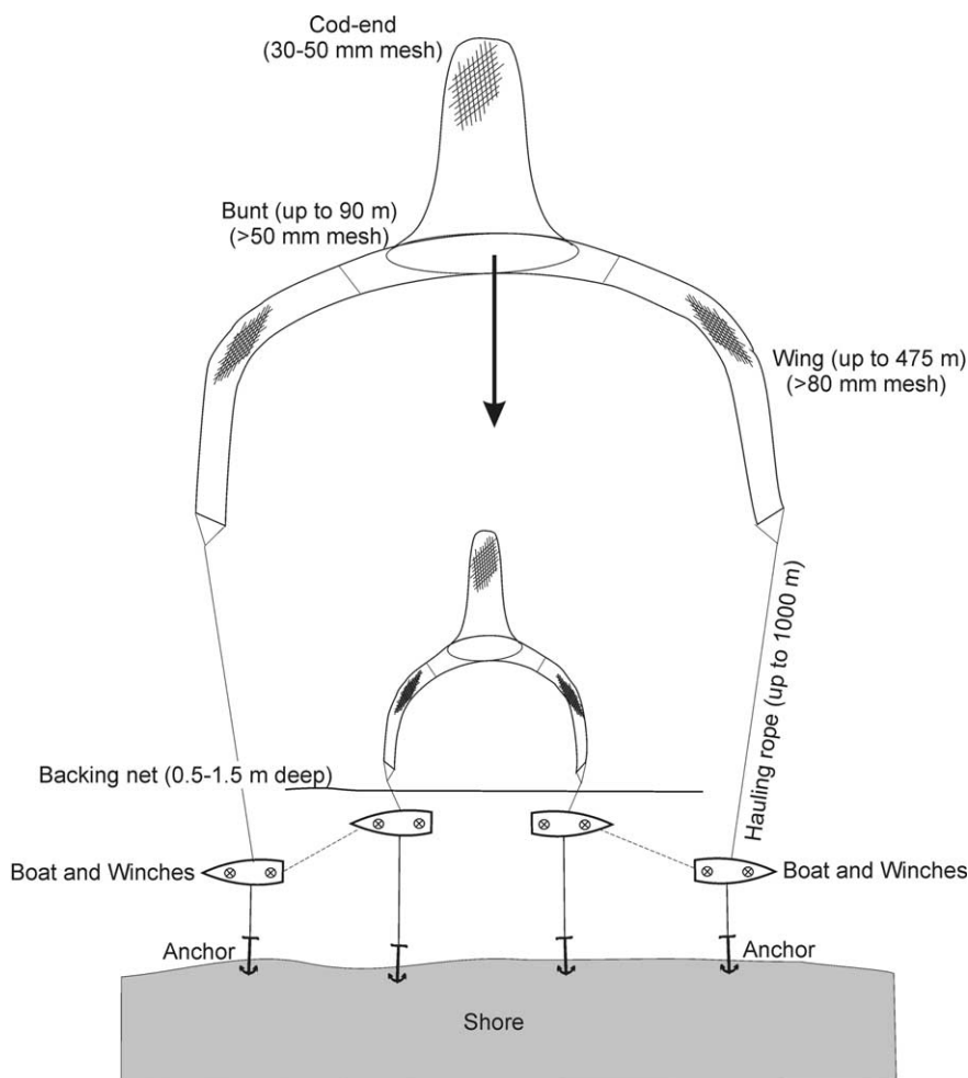
Fig. 2. Diagram of a beach-seine net as used in the NSW estuarine beach-seine fishery.
