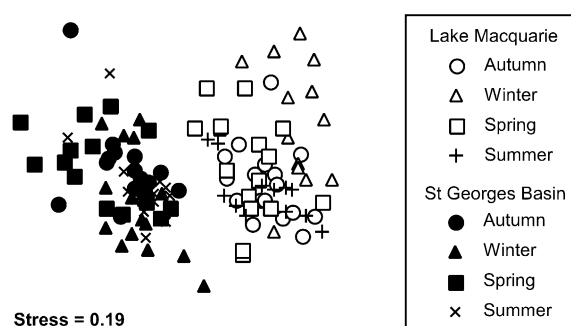
Fig. 3. MDS ordination showing differences in the assemblage composition of catches between estuaries based on numbers of each species captured.
